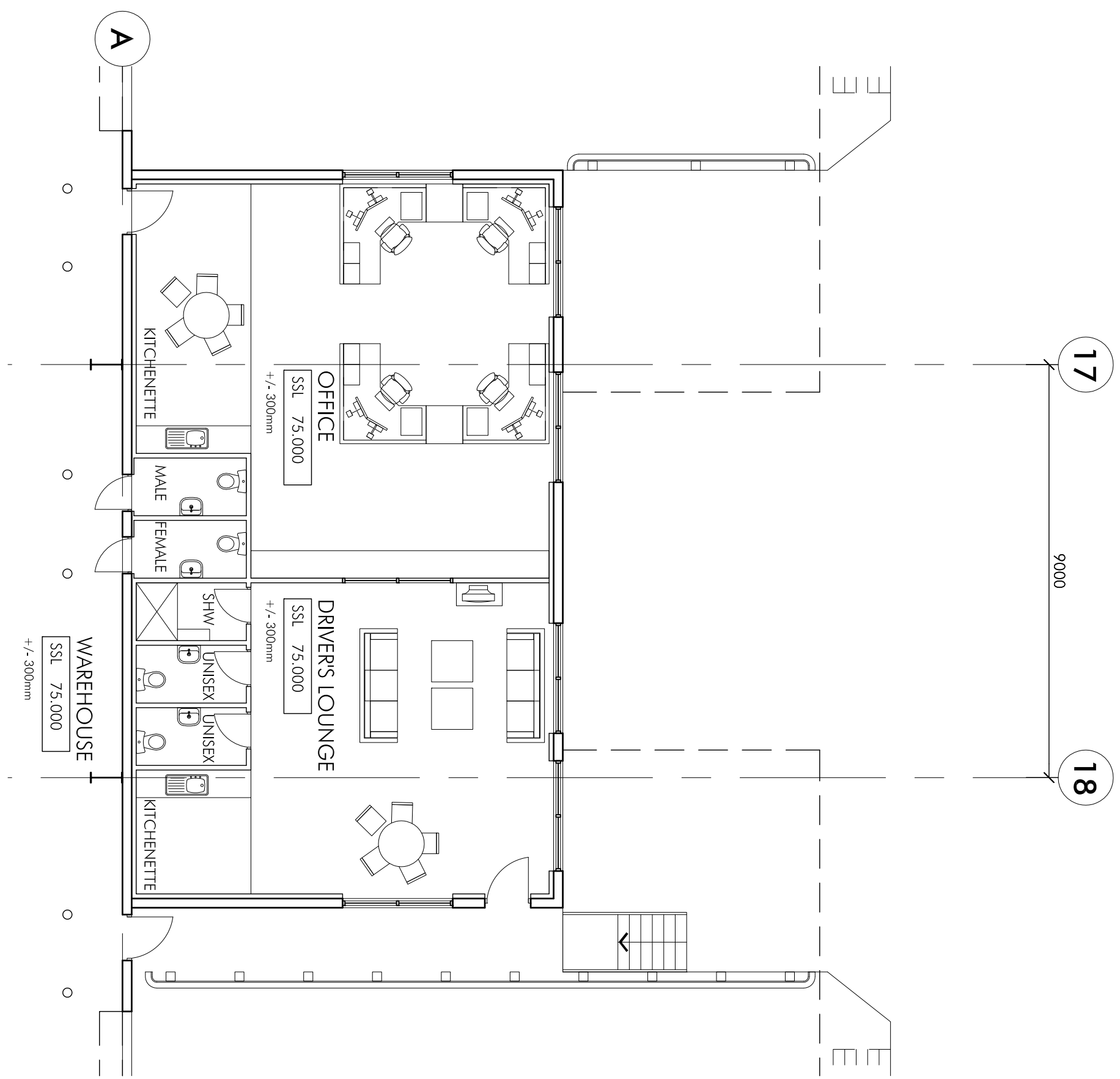
01. DOCK OFFICE & DRIVERS LOUNGE 1:100
